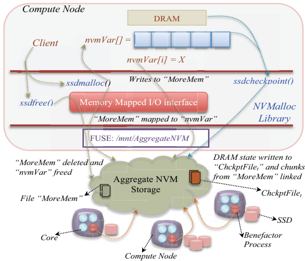
Figure 1. NVMMalloc overview
