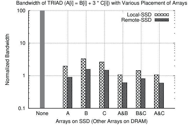
Figure 2. Bandwidth of STREAM TRIAD. Y-axis is normalized to show the bandwidth measured in the DRAM-only mode as 100. Note that a logarithmic scale is used for the Y-axis. X-axis shows which arrays are on the NVM. “None” indicates all arrays are on DRAM.
