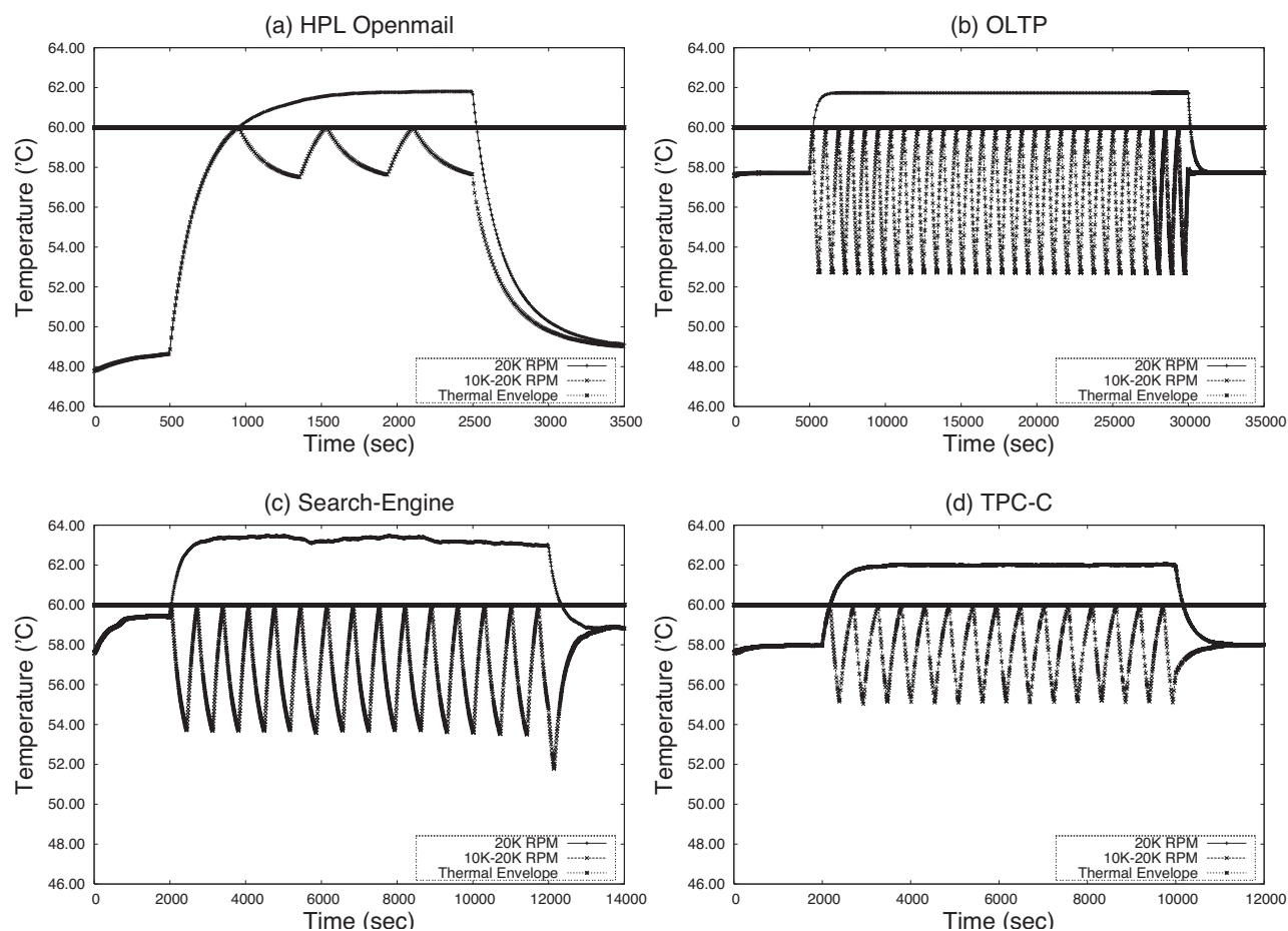
Fig. 5 Thermal profiles of the real workloads for DRPM opt under the scenarios of Table 1. They are all for the disk0 of disk arrays each of which is a 10–20 K multispeed disk with 7 s of RPM transition time and 400 s of a cooling unit time.
