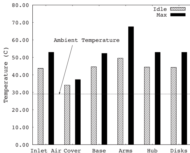
Fig. 2 Temperature distribution over IBM Ultrastar 146Z10. The dotted line denotes the ambient temperature (29°C). Each label in the X-axis indicates each component in the disk-drive. "Inlet Air" denotes external inlet air temperature. The description about all other labels can be found in Fig. 1(a).
