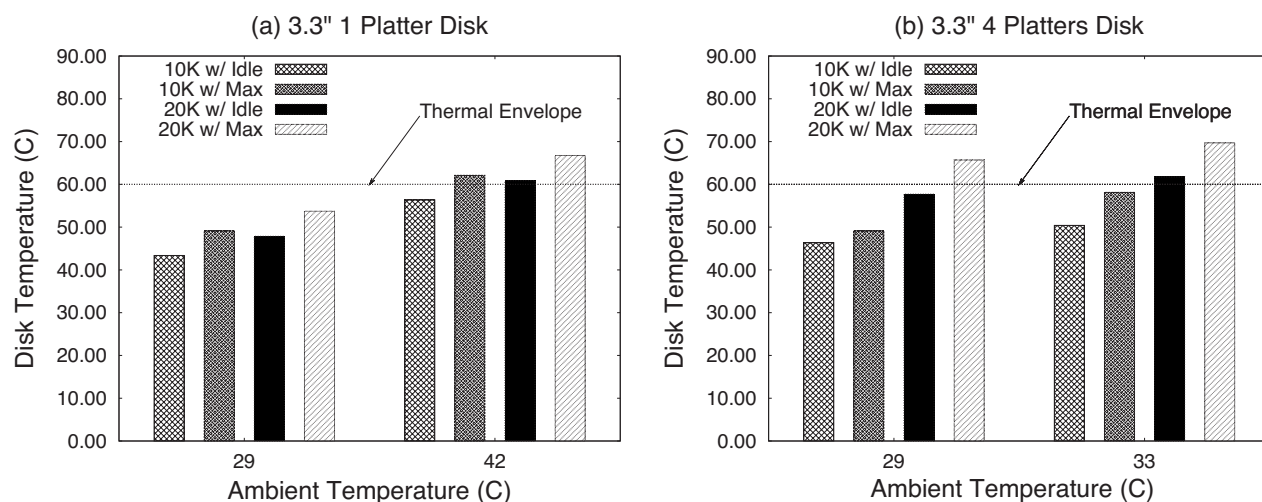
Fig. 3 Each bar denotes the average temperature of each component at the steady state for Max (where VCM is on all the times while the disk platters are spinning) and Idle (VCM just turns off). The horizontal line in each graph is the thermal envelope (60°C). (a) and (b) are the steady-state base temperatures of the disk for different disk dimensions (such as the size of platter and the rotational speed of platter) and different power consumption modes under various ambient temperatures. The horizontal line in each graph is the thermal envelope (60°C).
