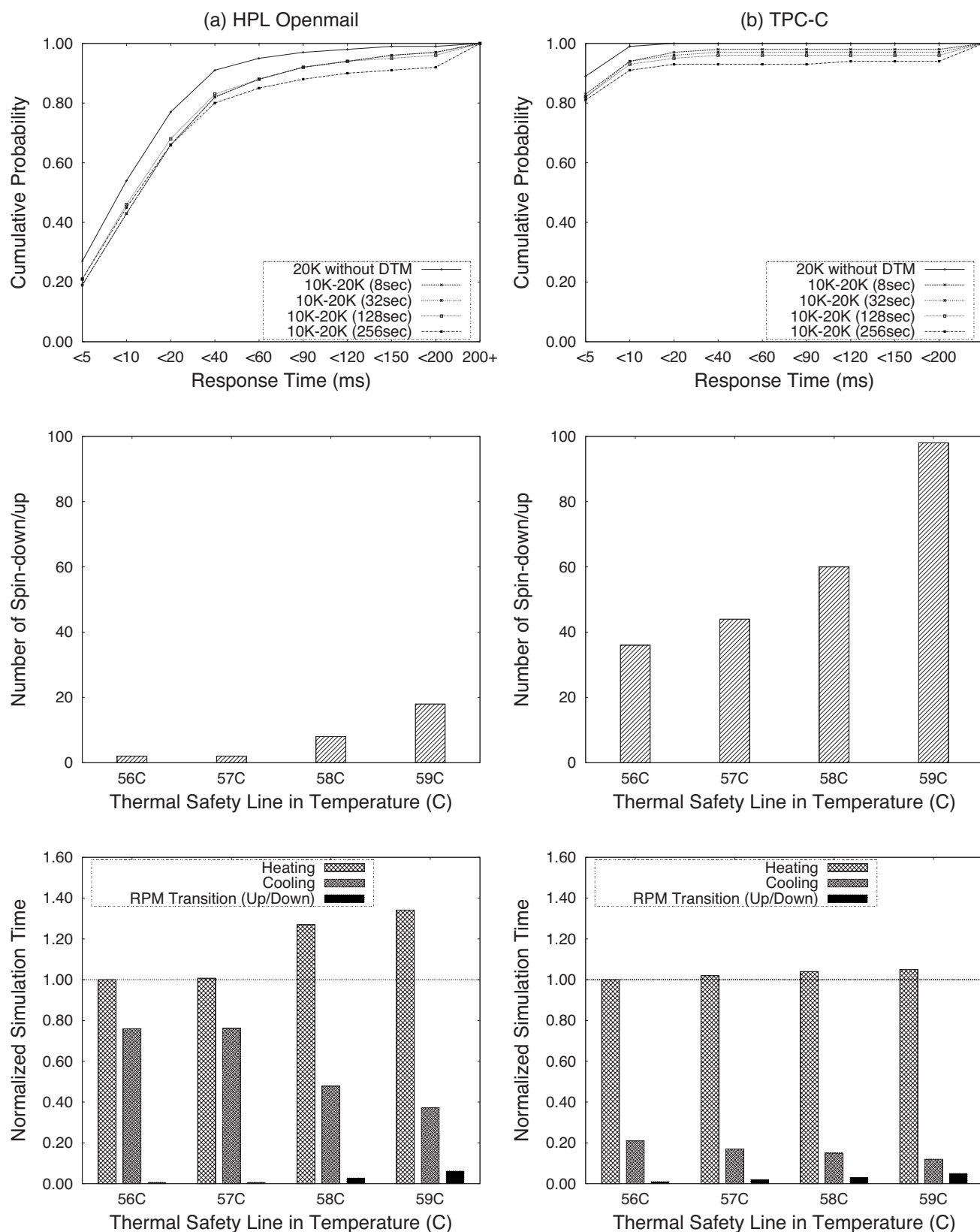
Fig. 7 Experimental results of DRPM opt using watermark-based policy for HPL Openmail and TPC-C. “Thermal Safety Line” in the graphs denotes temperature at which the disk-drive sufficiently cools down to operate.
