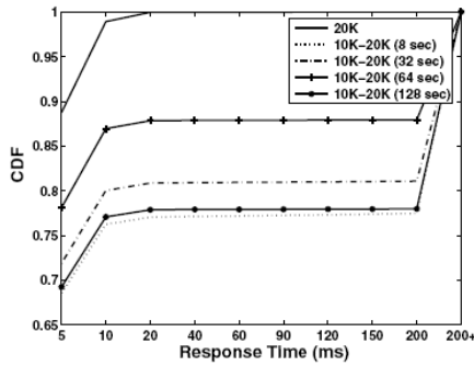
(b) TPC-C
