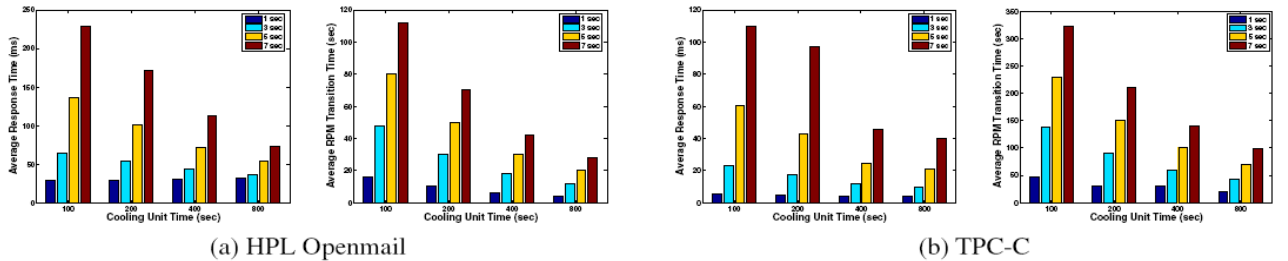
Figure 4. The first column for each workload is to understand the correlation between cooling unit time and RPM transition time. Each bar denotes an average response time across the disks at disk array in the unit of millisecond. And the second column for each workload denotes the average total time taken for RPM transitions across the disks in the unit of second.
