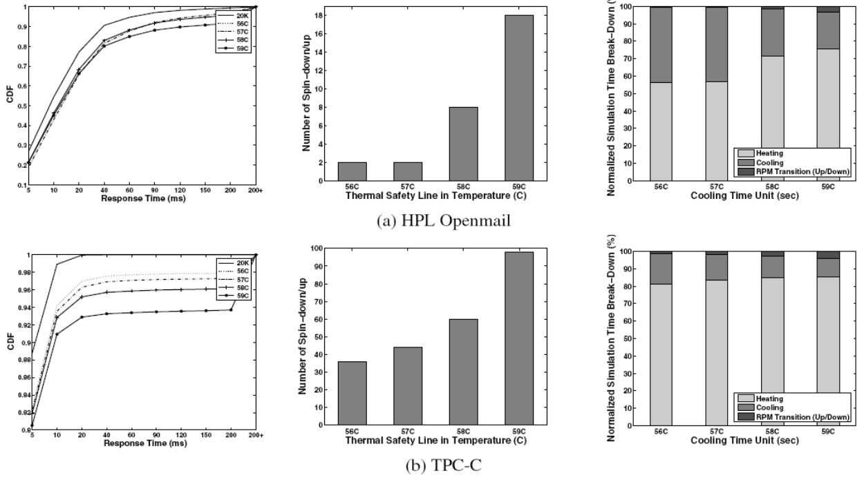
Figure 5. Experimental results of DRPM_{opt} using watermark-based policy for HPL Openmail and TPC-C
