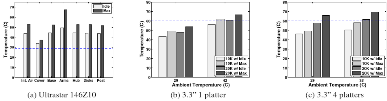
Figure 1. (a) shows temperature distribution of IBM Ultrastar 146Z10. Each bar denotes the average temperature of each component at the steady state for Max (where VCM is on all the times while the disk platters are spinning) and Idle (VCM just turns off). The dotted line denotes the ambient temperature (29°C). (b) and (c) are the steady-state base temperatures of disk for different disk dimensions (such as the size of platter and rotational speed of platter) and different power consumption modes under various ambient temperatures. The horizontal line in each graph is thermal envelope (60°C).
